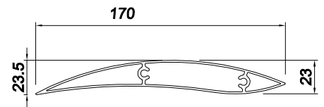
VINASTAR EX0000565 THK. 1.30 mm - 1.455 Kg/m
